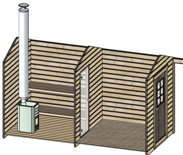
3D-vy insida
